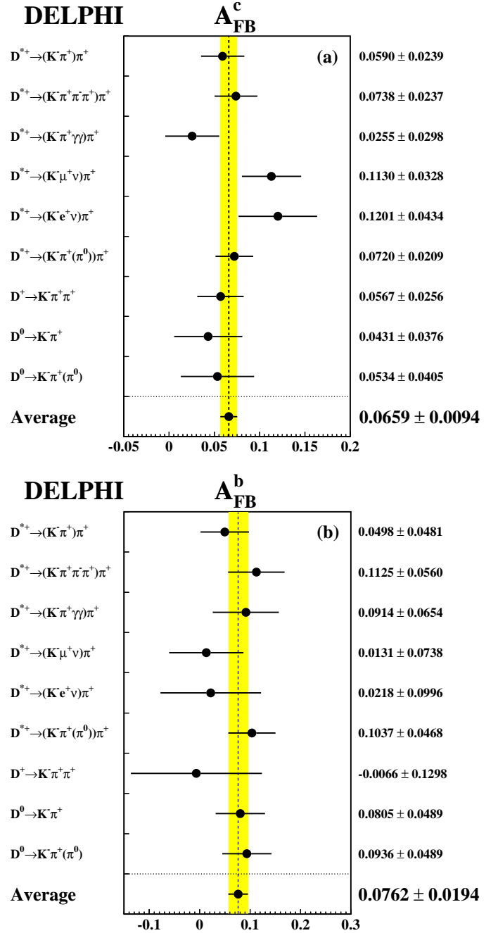
Fig. 4a,b. The results of the two parameter fit of the c and b asymmetry at an average centre-of-mass energy of 91.235 GeV for the different D samples are shown. The grey bands represent the averages over all these measurements. Only statistical errors are shown
