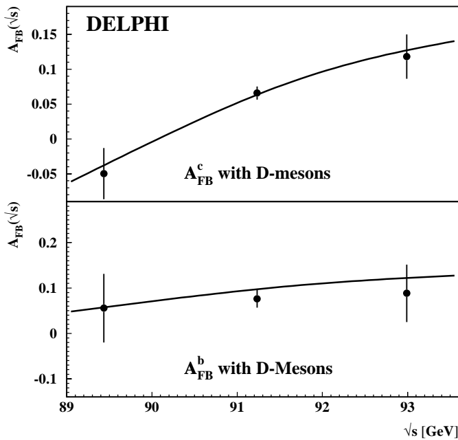
Fig. 8. The c and b forward–backward asymmetries for the different average centre–of–mass energies. The SM prediction is also shown ( M_Z = 91.187 \text{ GeV}/c^2 , m_{top} = 175.6 \text{ GeV}/c^2 , m_H = 300 \text{ GeV}/c^2 , \alpha_s(M_Z^2) = 0.120 , \alpha(M_Z^2) = 1/128.896 )
