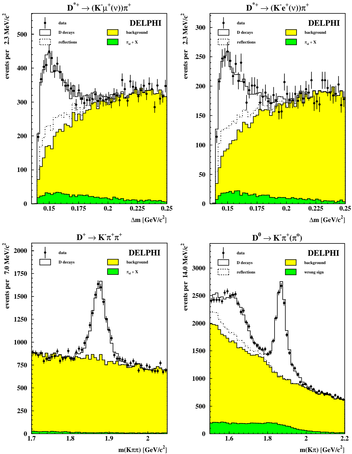
Fig. 2. The mass difference distributions \Delta m for the semileptonic decay modes are shown in the two upper plots. \Delta m is defined as the difference between the mass of the D^{*+} and the D^0 candidate. The data are compared to the simulation. Contributions from reflections, partially reconstructed D^{*+} decays and combinatorial background are also shown. The lower diagrams show the D^+ and D^0 mass distributions. For the D^0 the background distribution for candidates with wrong mass assignments is also shown. In the D^0 case, the peak in the K^- \pi^+ mass distribution comes from D^0 decays into K^- \pi^+ , and the broad enhancement at lower values is from the K^- \pi^+ \pi^0 decay
