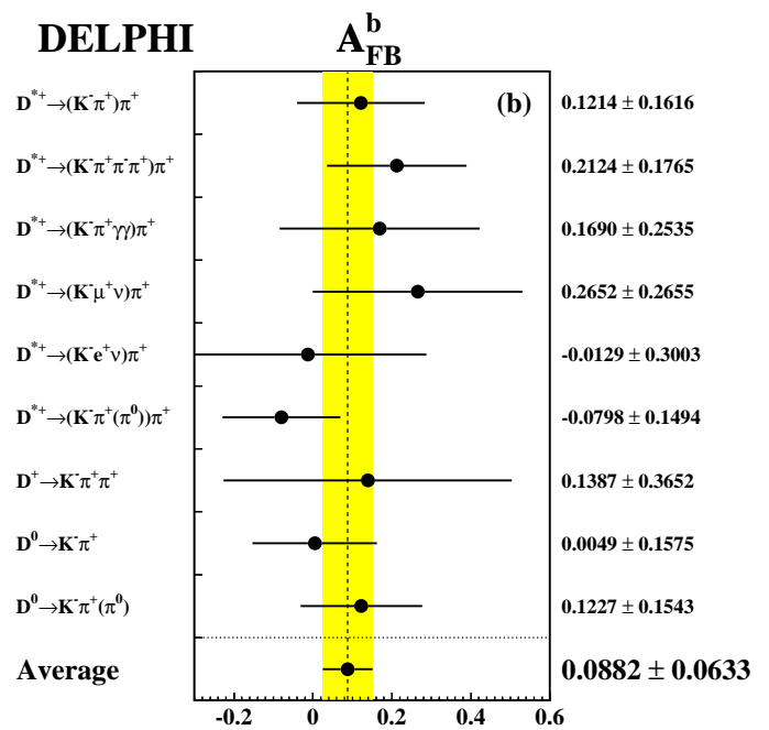
Fig. 7a,b. The results of the two parameter fit of the c and b asymmetry at an average centre-of-mass energy of 92.99 GeV for the different D samples are shown. The grey bands represent the averages over all these measurements. Only statistical errors are shown
