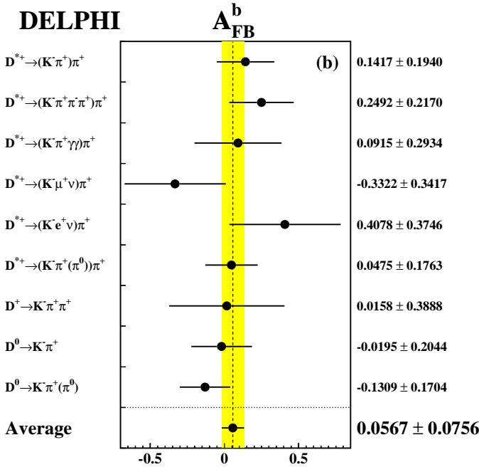
Fig. 6a,b. The results of the two parameter fit of the c and b asymmetry at an average centre-of-mass energy of 89.434 GeV for the different D samples are shown. The grey bands represent the averages over all these measurements. Only statistical errors are shown
