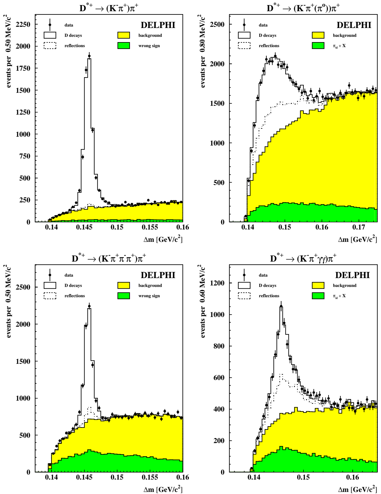
Fig. 1. The mass difference distributions \Delta m for the different decay modes. \Delta m is defined as the difference between the mass of the D^{*+} and the D^0 candidate. The data are compared to the simulation. Contributions from reflections, partially reconstructed D^{*+} decays ( \pi_{sl} + X ) and combinatorial background are also shown. See Sect. 5 for the discussion of these contributions
