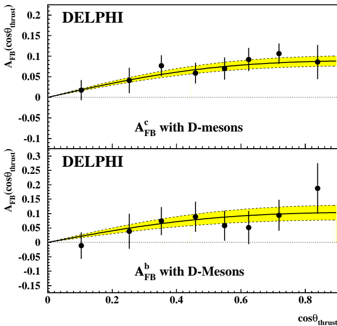
Fig. 5. The c and b forward-backward asymmetries at an average centre-of-mass energy of 91.235 GeV as a function of \cos \theta_{thrust} . Only statistical errors are shown. The bands represent the fit results
